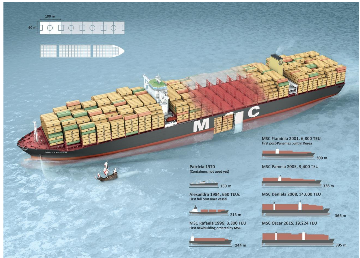
MSC OSCAR 2015, FULLY CELLULAR CONTAINER SHIP
